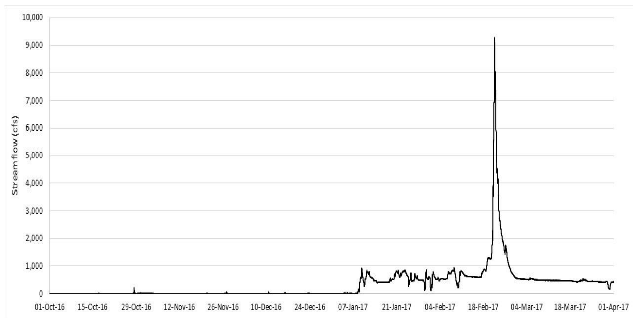
Figure 6. Mean daily stream flow at the SCVWD Edendale gage (in the urban area downstream of Metcalf Percolation Pond) from 1 October 2016 through 1 April 2017.
